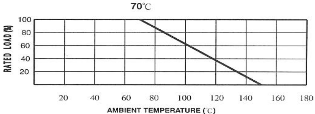
FIG.1 DERATING CURVE
